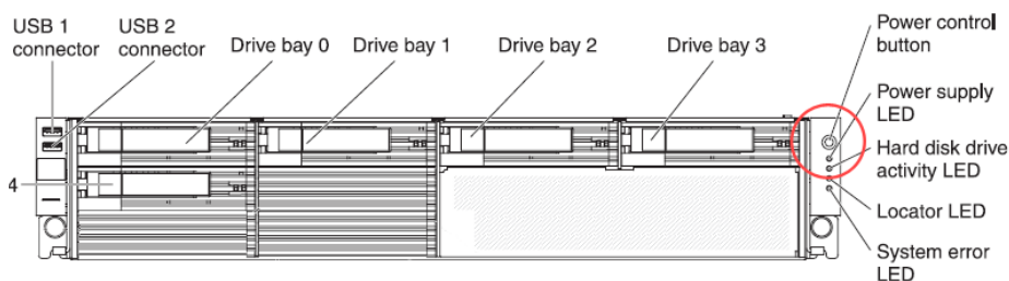
Fig. 7 - 705 / 735 model front panel, power button at far right
