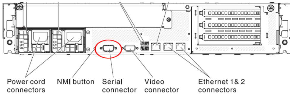
Fig. 4 - Rear of 705 / 735 model chassis, serial port circled in red
