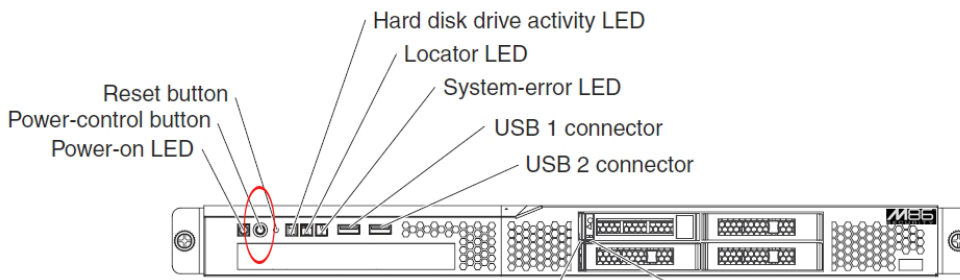
Fig. 9 - 505 model front panel, power button at far left
