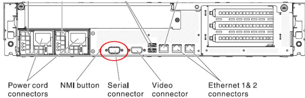
Fig. 5 - Rear of 705 / 735 model chassis, serial port circled in red
