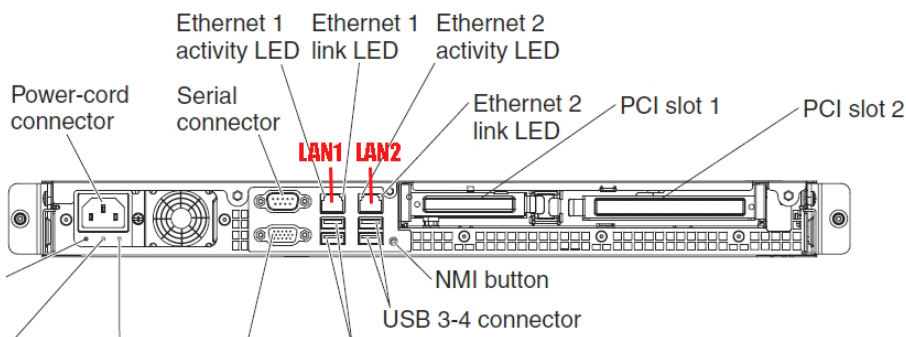
Portion of 505 model chassis rear with LAN ports identified
