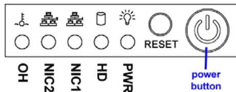
500 model chassis front panel
