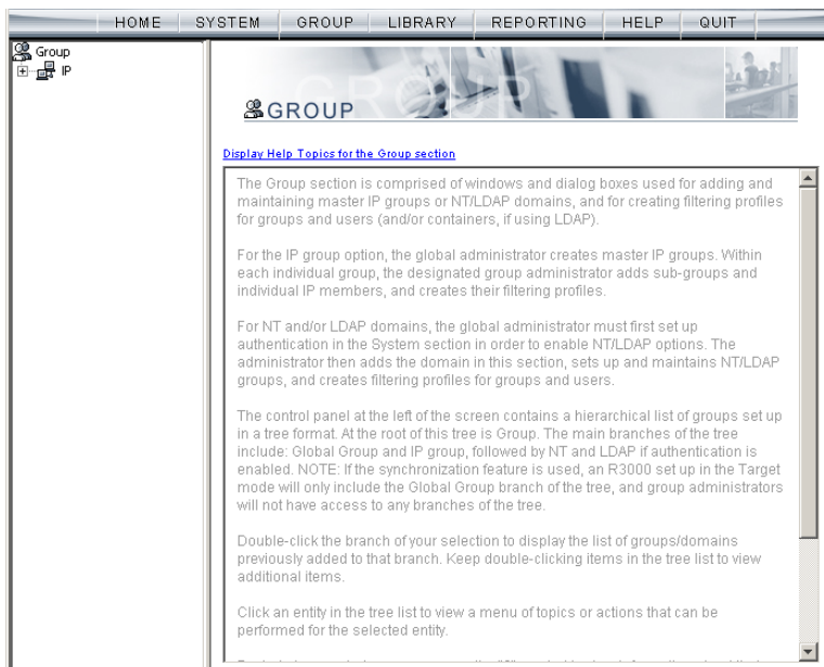
Fig. 3:1-1 Group screen
