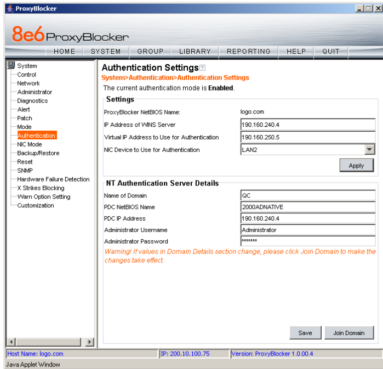
Fig. 3-1 Authentication Settings window
