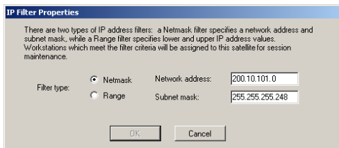
Fig. A-24 IP Filter Properties dialog box, Netmask
