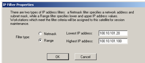
Fig. A-25 IP Filter Properties dialog box, Range
