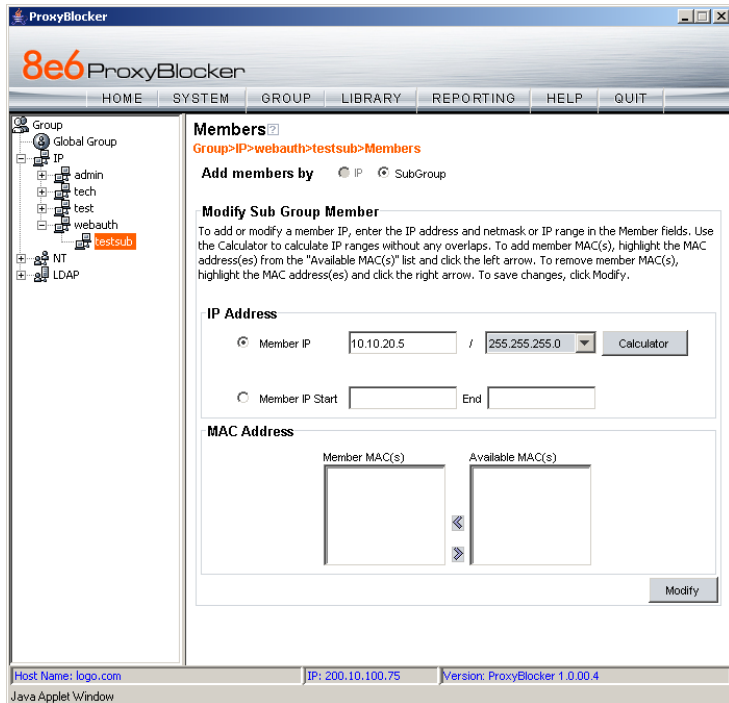
Fig. 5-14 Sub Group Members window
