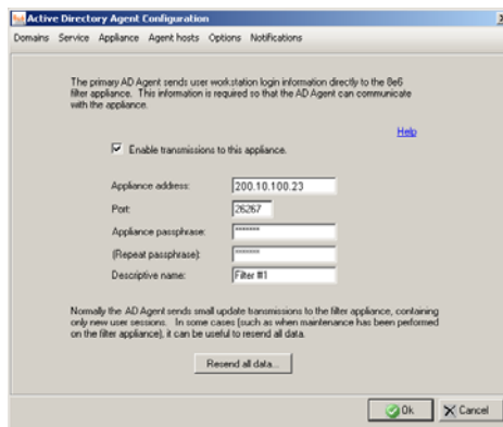
Fig. A-20 Primary host Configuration, Appliance
