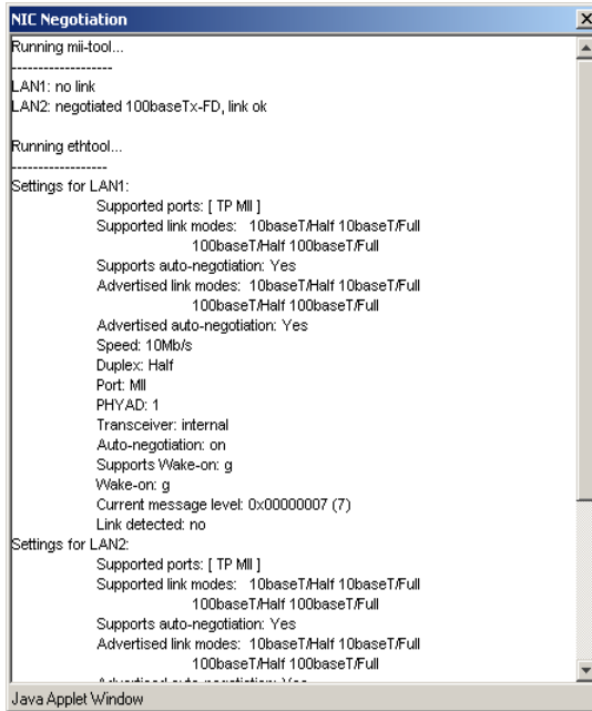
Fig. 2:1-70 NIC Negotiation window
