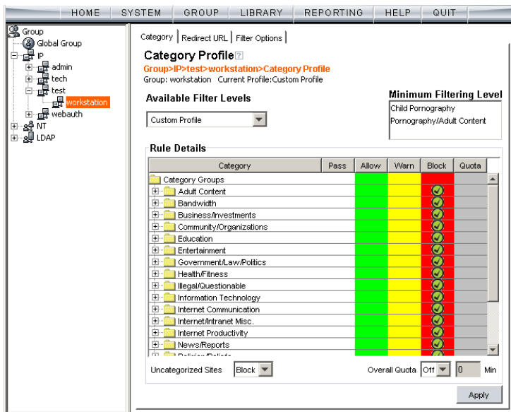
Fig. 6-6 Sub Group Profile window, Category tab
