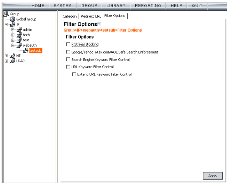
Fig. 6-17 Sub Group Profile window, Filter Options tab
