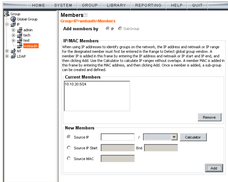
Fig. 6-12 Members window
