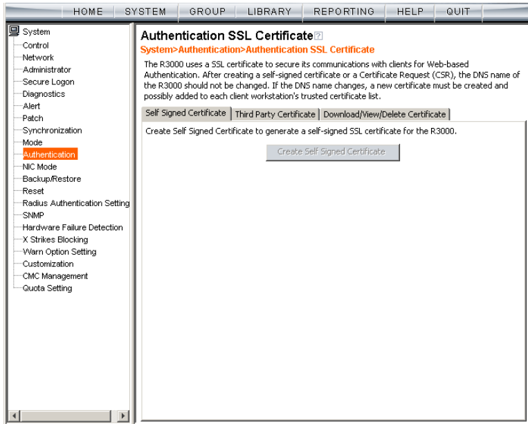
Fig. 2-7 Authentication SSL Certificate window
