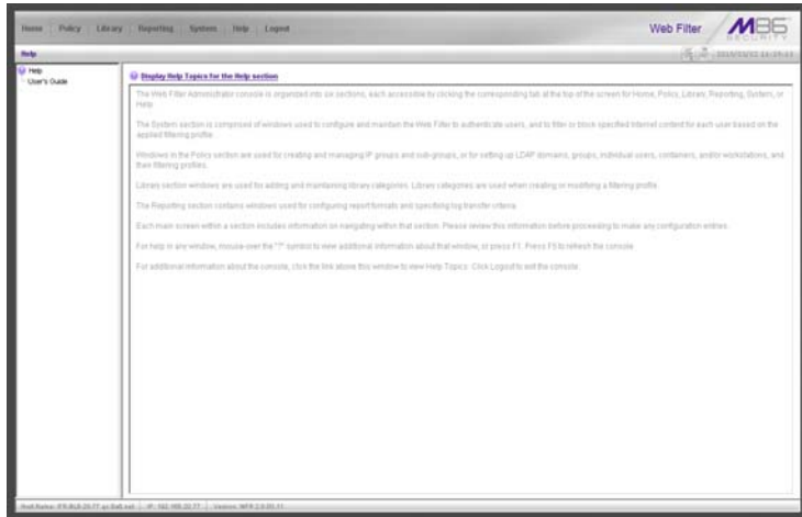
Fig. 1:4-5 Help screen
