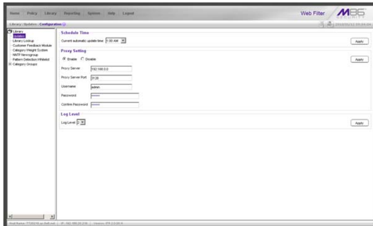
Fig. 2:3-2 Configuration window
