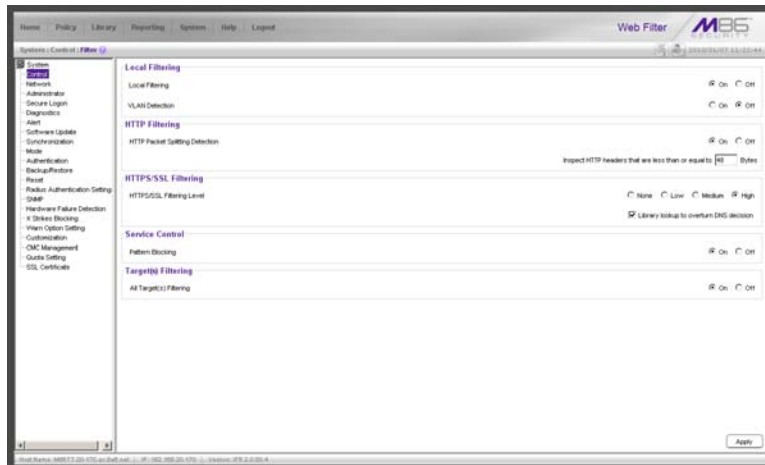
Fig. 2:1-2 Filter window
