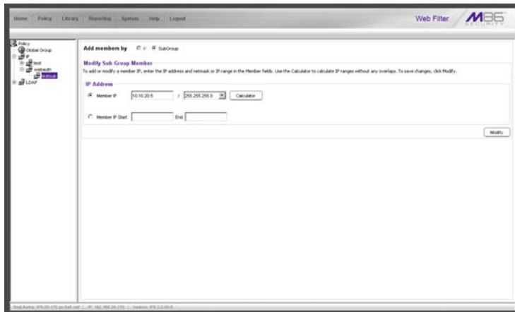
Fig. 5-14 Sub Group Members window
