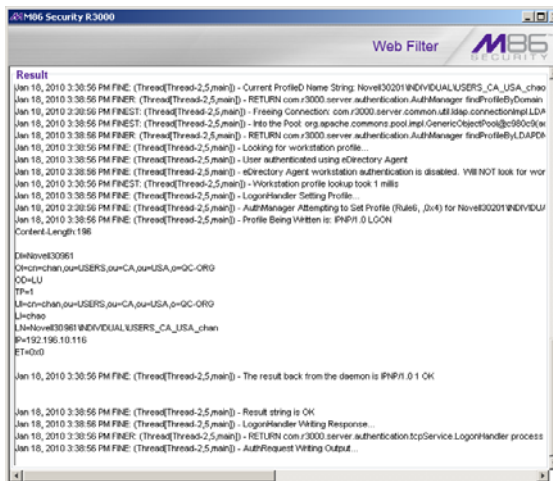
Fig. 2-25 View Log File Result window
